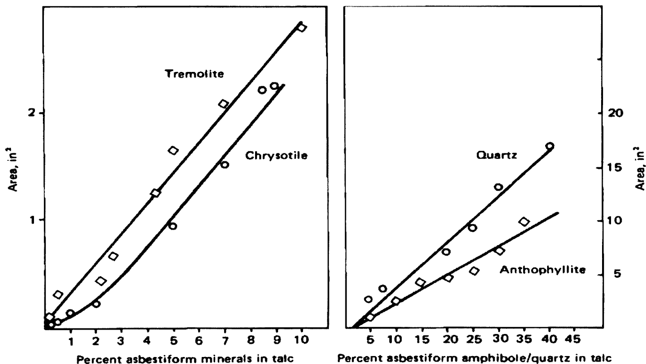
FIGURE 2. Calibration of asbestiform amphiboles and quartz in talc.
