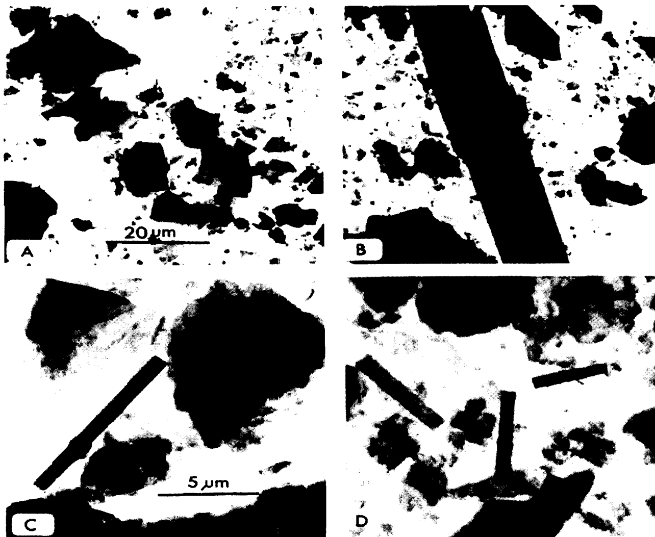
FIGURE 4. Transmission electron micrographs of cosmetic talc samples composed primarily of plates with an occasional large talc fiber (B, C); talc with many talc fibers (D); Scale is the same in (A) and (B) and in (C) and (D). All selected area electron diffraction patterns obtained on fibers yielded those consistent for talc plates (see Fig. 5, A and B). In all talc-containing samples examined by electron microscopy talc grains tended to range from 25 to 0.2 \mu\text{m} in greatest dimension. Micrograph obtained on a JEOL JEM 120 U with an acceleration voltage at 120 kV.
