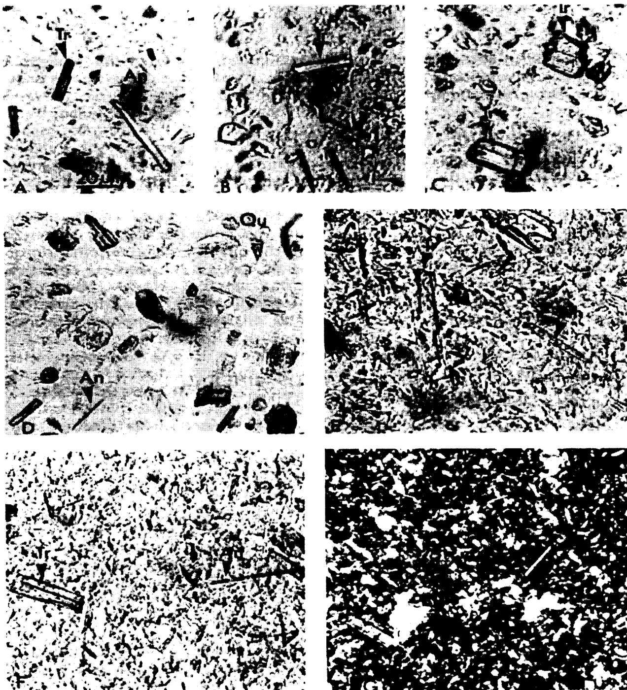
FIGURE 1. Optical photomicrographs of cosmetic talcums and powders grossly contaminated with asbestiform minerals. Photos obtained in plane polarized light (A-F) and between crossed polars (G). Scale in (A) for all photos. Fibers shown have optical properties consistent with tremolite (Tr) and anthophyllite (An). Quartz grains (Qu) and calcite fragments (Ca) are also shown. Most tremolite fibers tend to possess smaller length-to-width ratios than anthophyllite. Tremolite is observed as fragments (C). Photo obtained between crossed polars (G) also demonstrates the presence of fibers in the matrix material. Asbestiform length-to-width ratios measured up to 20:1 (F).
