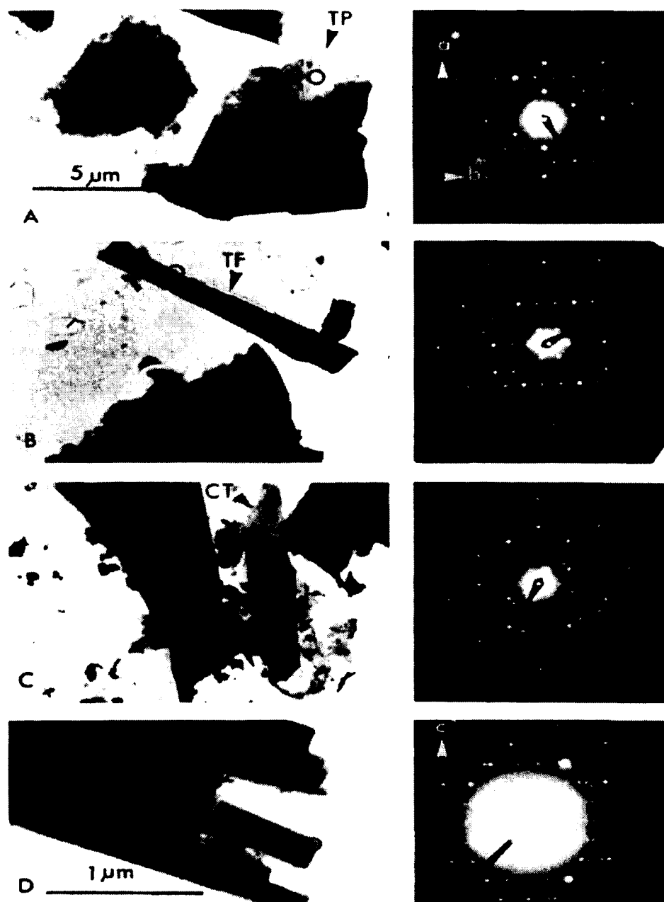
FIGURE 5. Transmission electron micrographs and accompanying selected area electron diffraction (SAED) patterns for cosmetic talc samples. The talc plate (TP) in (A) shows typical polygonal cleavage and diffraction contrast contours for the mineral species. The accompanying SAED pattern displays the characteristic reciprocal ab^* plane pseudo-hexagonal symmetry for talc. Talc a^* and b^* directions indicated on (A). Measurement of pattern indicates a 5.3 Å repeat along a^* and a 9.1 Å repeat for b^* (measured at [110] ). Talc fiber (TF) in (B) displays irregular ends and nonrectilinear edges. The SAED pattern is also pseudo-hexagonal, but some reflection intensities [e.g., the (060), (0.12.0)] are more pronounced. This may be due to both orientation and structural effects. The curled talc plate (CT) in (C) displays an incipient Debye-Scherrer ring pattern (the effects of both folding over of talc and small associated grains). The amphibole fiber (D) was diffracted only on one of the protruding unit fibrils. The c^* axis is shown, with repeat measured at 5.3 Å. Areas where diffraction patterns were obtained are indicated by location circles; particles were photographed at the SAED magnification \times 26,500 . Scale is the same in A-C; scale in D as marked. Micrographs obtained on a JEOL JEM 120U with an accelerating voltage at 120 kV.
