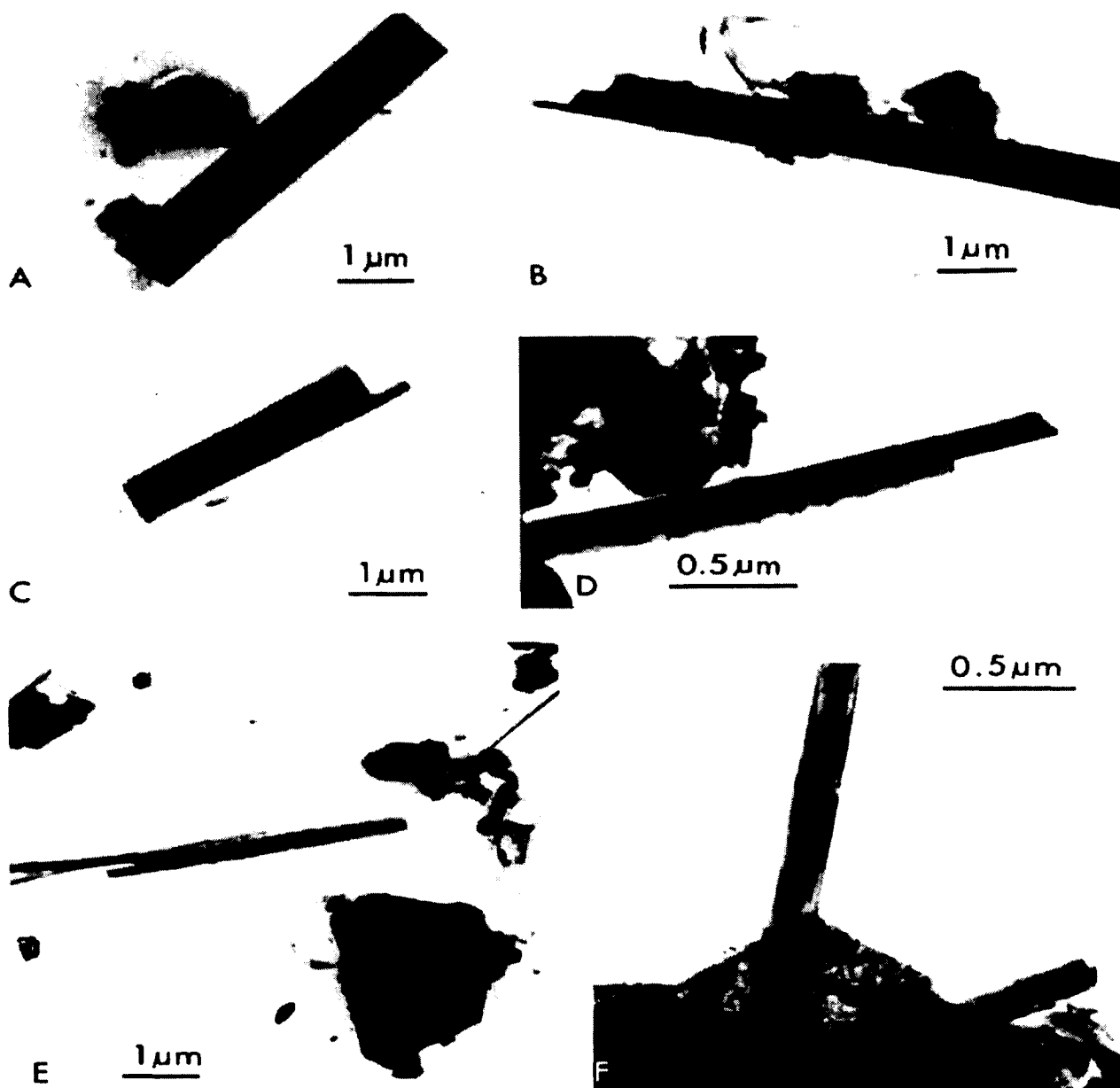
FIGURE 3. Transmission electron micrographs showing range in morphological characteristics of asbestiform tremolite and anthophyllite in talc. The entire range of morphological variations observed for these minerals is observed in the asbestos standards: rectilinear fibers with parallel ends and edges (A); step-cleavage ends (B); unit fibrils protruding from fiber body, (C); curvilinear fiber with amphibole cleavage end (D); high length-to-width ratio fibers (E); fibers protruding from interiors of talc plates (F). All of these morphological variations and forms (A-E) have been described in anthophyllite and tremolite asbestos samples. The amphibole structure was confirmed in all cases by selected area electron diffraction characterization. Scale as marked. Micrographs obtained on a JEOL JEM 120 U with an accelerating voltage at 120 kV.
